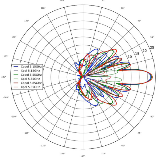
3 GHz Azimuth
