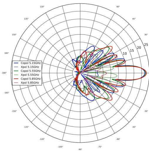
5 GHz Azimuth
