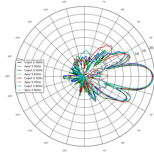
3 GHz Elevation
