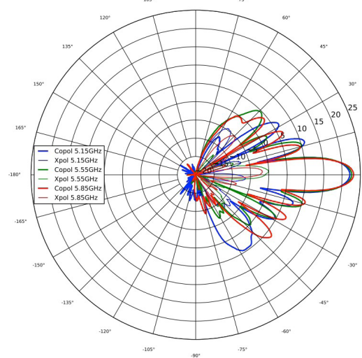
5 GHz Elevation
